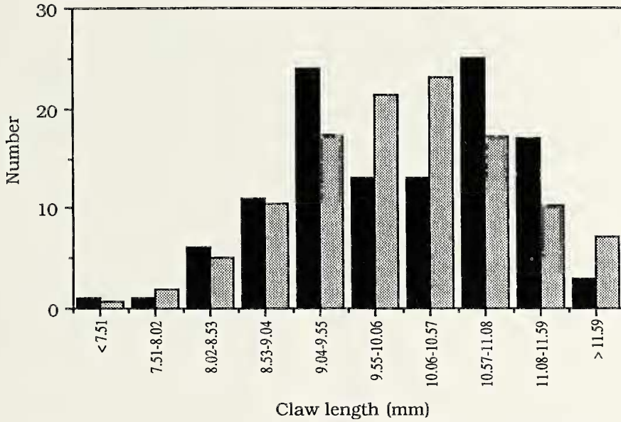
Figure 3.—The observed (filled bars) and expected (stippled bars) distributions of chela-lengths of 114 male scorpions from Sheerness. The expected distribution is a normal distribution given the mean and standard deviation of the observed. The distributions differ significantly ( \chi^2 = 21.1 , df = 7 , P < 0.001 ). The two modes of the observed distribution correspond to two instars.
